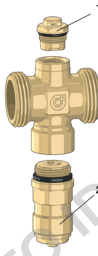
Valvola antigelo 108..2
