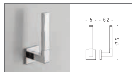
B3790 Porta rotolo Paper holder
