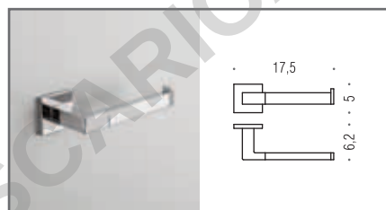
B3708DX Porta rotolo destro Right paper holder
